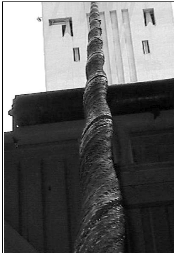
Figure 12: Deformation of the kibble ropes
