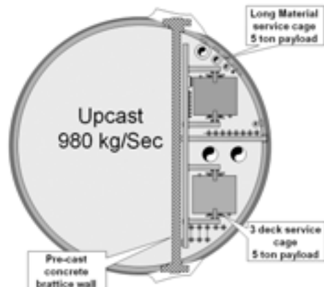
Figure 5: Ventilation Shaft
