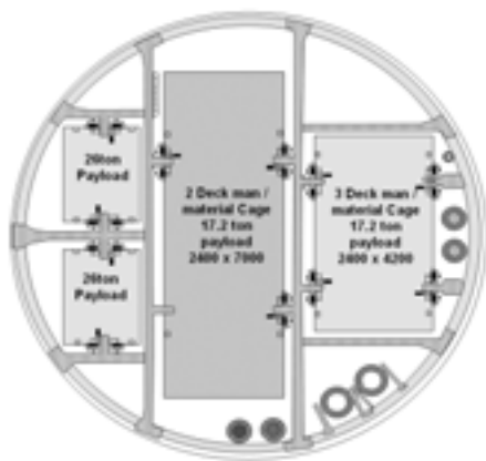
Figure 4: Main Shaft
