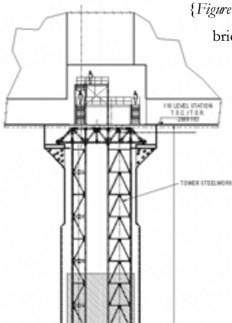
Figure 19: Side view of the Steel Tower
