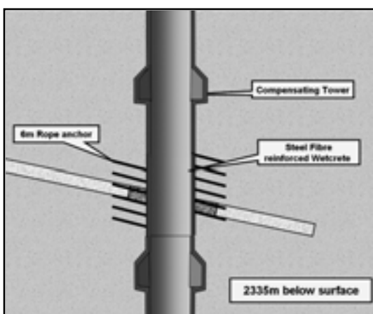
Figure 18: Schematic of secondary support used
